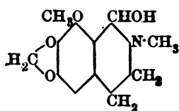
Cotarnine.
